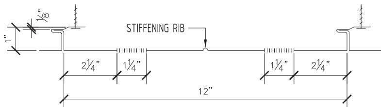
SINGLE BEAD – VENTED PROFILE
