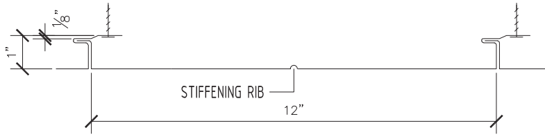
SINGLE BEAD – SOLID PROFILE
