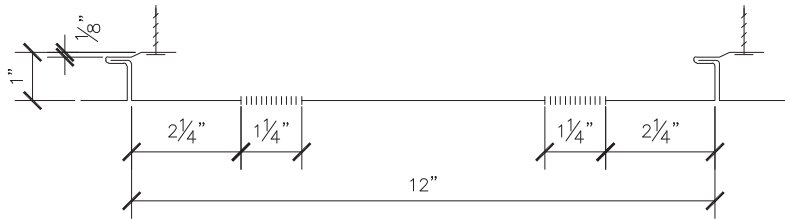
SMOOTH – VENTED PROFILE
