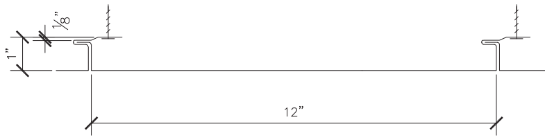
SMOOTH – SOLID PROFILE
