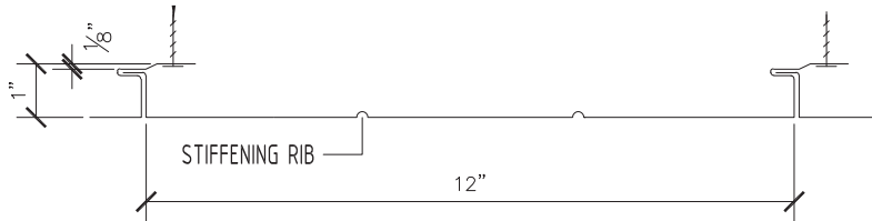
DOUBLE BEAD – SOLID PROFILE
