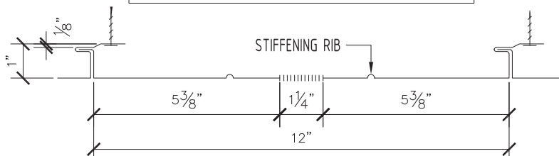
DOUBLE BEAD – VENTED PROFILE
